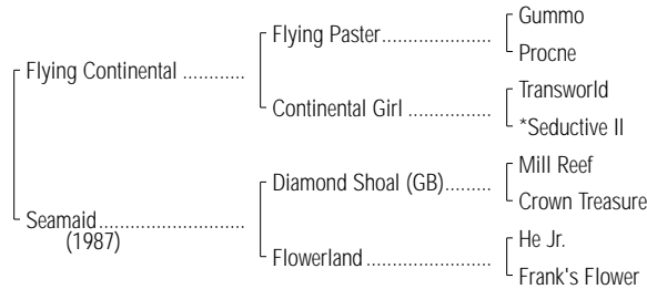
FLYING SEAMAID
